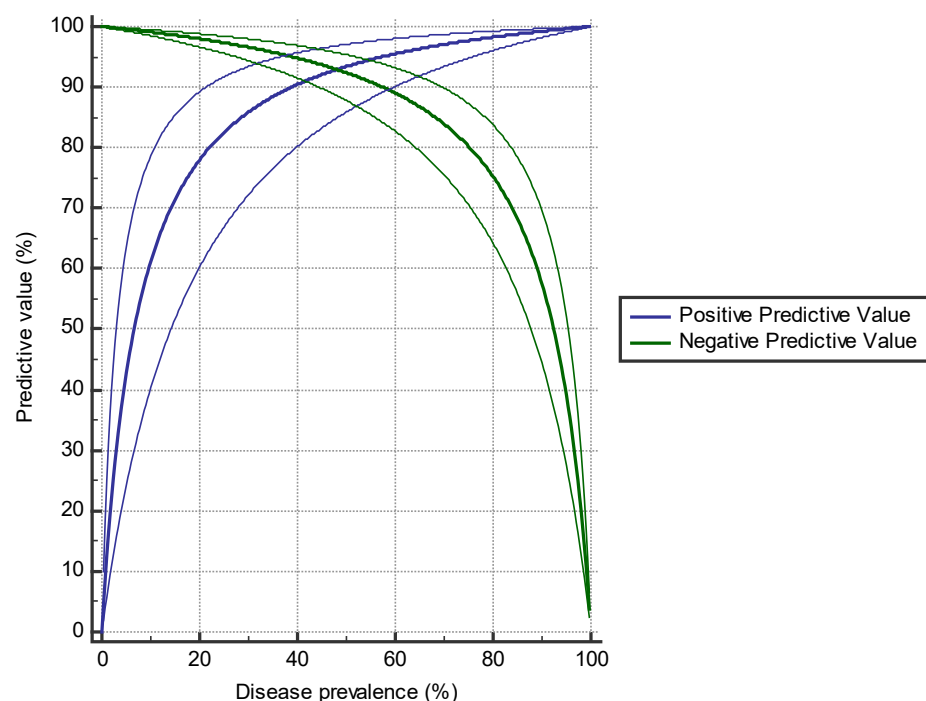
Fig. 1. Positive Predictive Value (PPV) and Negative Predictive Value (NPV) in relation to prevalence. The lower the prevalence the higher the NPV and the lower the PPV. The higher the prevalence the lower the NPV and the higher the PPV (test sensitivity 92.3% and specificity 93.5%, thin lines represent 95% confidence intervals and bold lines are point estimates of PV [https://www.medcalc.org/]).
